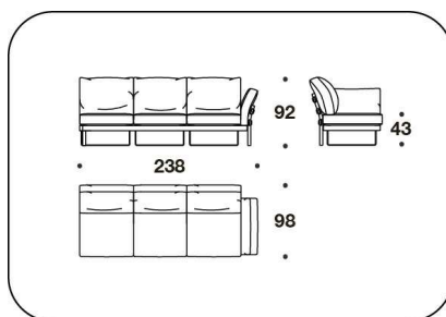
TOA (AE3D) - TOA (AE3S) ELEMENTO 3 POSTI C/BRACCIOLO DX O SX / 3 SEAT ELEMENT W/ARM RIGHT OR LEFT 238x98x92H. - H.S.43cm 93 2/3x38 2/3x36 1/3H. - H.S.17"
