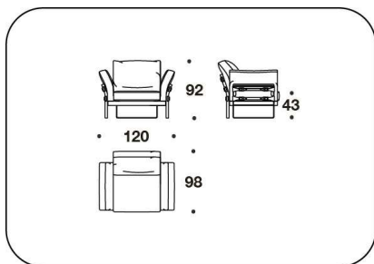
TOA (APOL) POLTRONA / ARMCHAIR 120x98x92H. - H.S.43cm 47 1/3x38 2/3x36 1/3H. - H.S.17"
