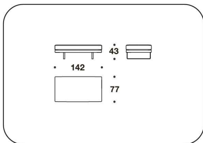
TOA (APOU3) POUF RETTANGOLARE / RECTANGULAR OTTOMAN 142x77x43H.cm 56x30 1/3x17H."
