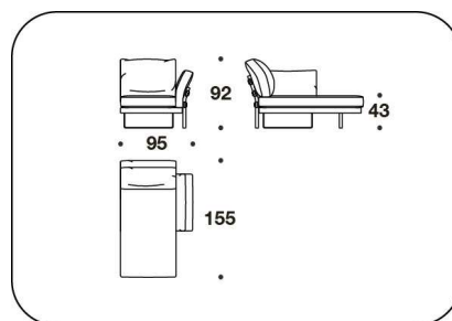
TOA (ACLD) - TOA (ACLS) CHAISE LONGUE : DX O SX / RIGHT OR LEFT 95x155x92H. - H.S.43cm 37 1/3x61x36 1/3H. - H.S.17"
