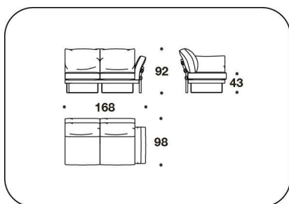
TOA (AE2D) - TOA (AE2S) ELEMENTO 2 POSTI C/BRACCIOLO DX O SX / 2 SEAT ELEMENT W/ARM RIGHT OR LEFT 168x98x92H. - H.S.43cm 66x38 2/3x36 1/3H. - H.S.17"
