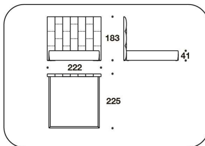
ASR (KUSA) KING USA : LETTO PER MATERASSO / BED FOR MATTRESS 195x205 - 222x225x183H. - H.B.41cm 76 2/3x80 2/3 - 87 1/3x88 2/3x72H. - H.B.16 1/4"
