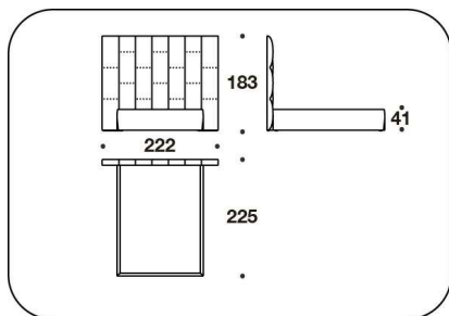
ASR (QUSA) QUEEN USA : LETTO PER MATERASSO / BED FOR MATTRESS 152x205 - 222x225x183H. - H.B.41cm 60x80 2/3 - 87 1/3x88 2/3x72H. - H.B.16 1/4"
