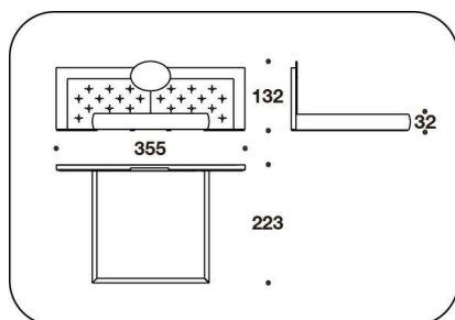
CME (LE7) LETTO PER MATERASSO / BED FOR MATTRESS 200x200 - 355x223x132H. - H.B.32cm 78 2/3x78 2/3 - 140x87 2/3x52H. - H.B.12 2/4"
