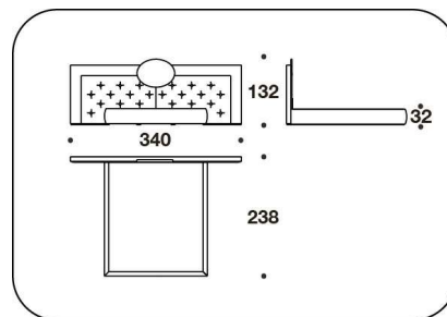
CME (CUSA) CALIFORNIA USA : LETTO PER MATERASSO / BED FOR MATTRESS 183x215 - 340x238x132H. - H.B.32cm 72x84 2/3 - 134x93 2/3x52H. - H.B.12 2/4"
