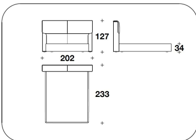
KIA (RLE1) CHESTNUT - BURR WALNUT : LETTO PER MAT. / BED FOR MATTRESS 165x200 - 202x233x127H. - H.B. 34cm 65x78 2/3 - 79 2/3x91 2/3x50H. - H.B. 13 2/4"
