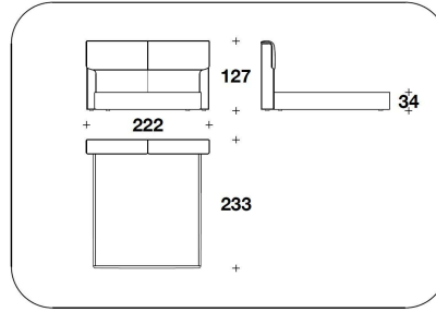
KIA (LE2) LETTO PER MATERASSO / BED FOR MATTRESS 185x200 - 222x233x127H. - H.B.34cm 73x78 2/3 - 87 1/3x91 2/3x50H. - H.B.13 2/4"
