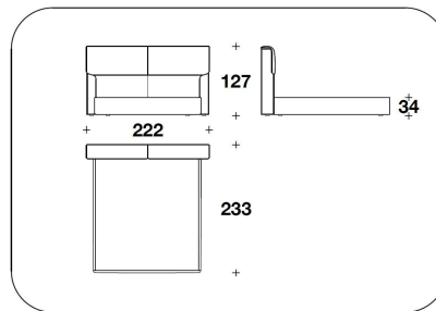
KIA (RLE2) CHESTNUT - BURR WALNUT : LETTO PER MAT. / BED FOR MATTRESS 185x200 - 222x233x127H. - H.B. 34cm 73x78 2/3 - 87 1/3x91 2/3x50H. - H.B. 13 2/4"
