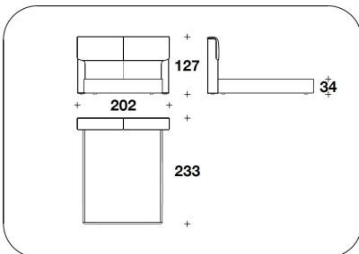
KIA (ELE1) EBONY MACASSAR : LETTO PER MAT. / BED FOR MATTRESS 165x200 202x233x127H. - H.B. 34cm 65x78 2/3 79 2/3x91 2/3x50H. - H.B. 13 2/4"
