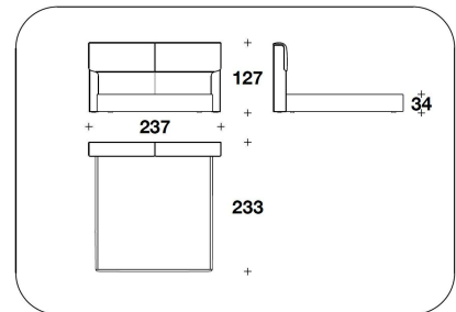
KIA (ELE7) EBONY MACASSAR : LETTO PER MAT. / BED FOR MATTRESS 200x200 237x233x127H. - H.B. 34cm 78 2/3x78 2/3 93 1/3x91 2/3x50H. - H.B. 13 2/4"
