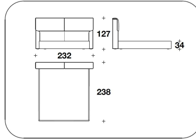
KIA (EKUSA) EBONY MACASSAR / KING USA : LETTO PER MAT. / BED FOR MATTRESS 195x205 232x238x127H. - H.B. 34cm 76 2/3x80 2/3 91 1/3x93 2/3x50H. - H.B. 13 2/4"
