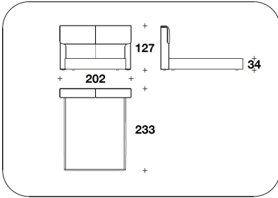
KIA (LE1) LETTO PER MATERASSO / BED FOR MATTRESS 165x200 - 202x233x127H. - H.B.34cm 65x78 2/3 - 79 2/3x91 2/3x50H. - H.B.13 2/4"
