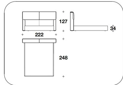
KIA (RCUSA) CHESTNUT - BURR WALNUT / CALIFORNIA USA : LETTO PER MAT. / BED FOR MATTRESS 183x215 - 222x248x127H. - H.B. 34cm 72x84 2/3 - 87 1/3x97 2/3x50H. - H.B. 13 2/4"
