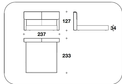
KIA (RLE7) CHESTNUT - BURR WALNUT : LETTO PER MAT. / BED FOR MATTRESS 200x200 - 237x233x127H. - H.B. 34cm 78 2/3x78 2/3 - 93 1/3x91 2/3x50H. - H.B. 13 2/4"
