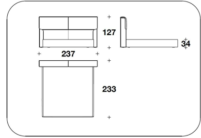
KIA (LE7) LETTO PER MATERASSO / BED FOR MATTRESS 200x200 - 237x233x127H. - H.B.34cm 78 2/3x78 2/3 - 93 1/3x91 2/3x50H. - H.B.13 2/4"
