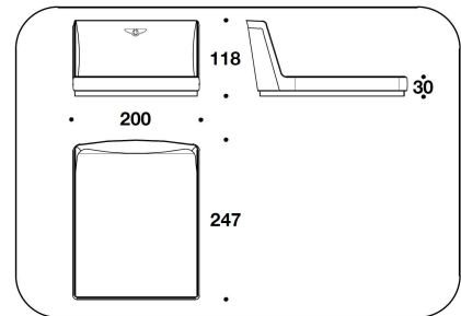
CNC (RCUSA) CHESTNUT - BURR WALNUT / CALIFORNIA USA : LETTO PER MATERASSO / BED FOR MATTRESS 183x215 - 200x247x118H. - H.B.30cm 72x84 2/3 - 78 2/3x97 1/3x46 1/3H. - H.B.11 3/4"
