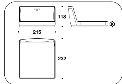
CNC (LLE7) LETTO LACCATO PER MATERASSO / LACQUERED BED FOR MATTRESS 200x200 - 215x232x118H. - H.B.30cm 78 2/3x78 2/3 - 84 2/3x91 1/3x46 1/3H. - H.B.11 3/4"
