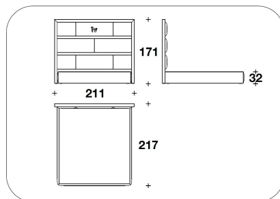
ZFR (LE2) LETTO PER MATERASSO / BED FOR MATTRESS 185x200 - 211x217x171H. - H.B.32cm 73x78 2/3 - 83x85 1/3x67 1/3H. - H.B.12 2/4"
