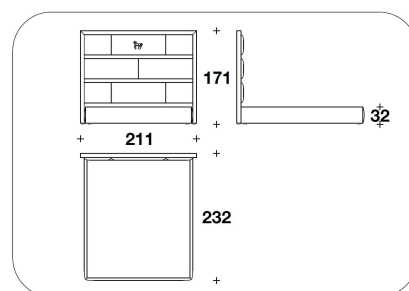
ZFR (CUSA) CALIFORNIA USA : LETTO PER MATERASSO / BED FOR MATTRESS 183x215 - 211x232x171H. - H.B.32cm 72x84 2/3 - 83x91 1/3x67 1/3H. - H.B.12 2/4"
