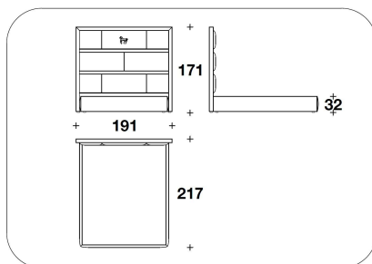
ZFR (LE1) LETTO PER MATERASSO / BED FOR MATTRESS 165x200 - 191x217x171H. - H.B.32cm 65x78 2/3 - 75 1/3x85 1/3x67 1/3H. - H.B.12 2/4"
