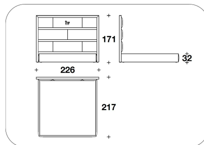
ZFR (LE7) LETTO PER MATERASSO / BED FOR MATTRESS 200x200 - 226x217x171H. - H.B.33cm 78 2/3x78 2/3 - 89x85 1/3x67 1/3H. - H.B.13"
