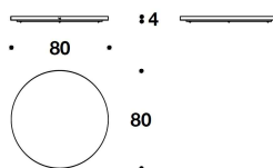
LVA (8L) - LVA (8E) LOTUS : VASSOIO / TRAY Ø 80x4H.cm Ø 31 1/3x1 9/16H."
