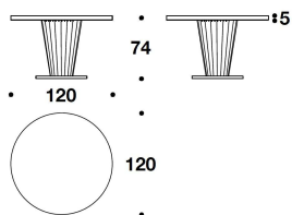
TVL (34L) - TVL (34M) - TVL (34I) TAVOLO TONDO / ROUND TABLE Ø 120x74H. - THK.5 / THK.2cm Ø 47 1/3x29H. - THK.1 15/16 / THK.0 13/16"
