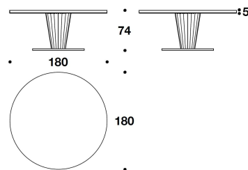
TVL (32L) - TVL (32M) - TVL (32I) TAVOLO TONDO / ROUND TABLE Ø 180x74H. - THK.5 / THK.2cm Ø 71x29H. - THK.1 15/16 / THK.0 13/16"
