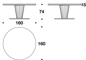
TVL (33L) - TVL (33M) - TVL (33I) TAVOLO TONDO / ROUND TABLE Ø 160x74H. - THK.5 / THK.2cm Ø 63x29H. - THK.1 15/16 / THK.0 13/16"
