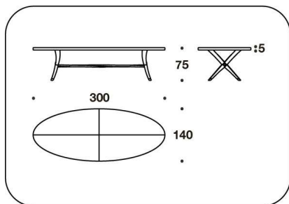
TAV (T64P) - TAV (T64E) - TAV (T64R) - TAV (T64RA) TAVOLO OVALE / OVAL TABLE 300x140x75H. - THK.5cm 118x55x29 2/3H. - THK.1 15/16"
