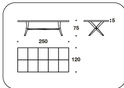
TAV (T62P) - TAV (T62E) - TAV (T62R) - TAV (T62RA) TAVOLO RETTANGOLARE / RECTANGULAR TABLE 250x120x75H. - THK.5cm 98 1/3x47 1/3x29 2/3H. - THK.1 15/16"
