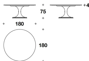
TTV (15LP) TAVOLO / TABLE Ø 180x75H. - THK.4cm Ø 71x29 2/3H. - THK.1 9/16"
