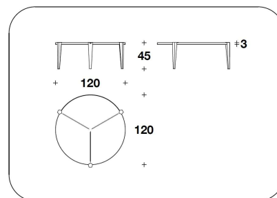
TCT (CF60/3) - TCT (CF60/2) - TCT (CF60/1) COFFEE TABLE Ø 60x32H. - 90x39H. - 120x45H.cm Ø 23 2/3x12 2/4H. - 35 1/3x15 1/4H. - 47 1/3x17 3/8"
