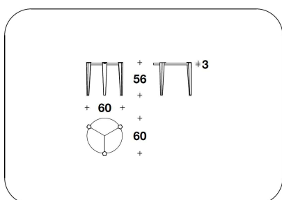
TCT (CF61/1) SIDE TABLE Ø 60x55H.cm Ø 23 2/3x21 2/3H."
