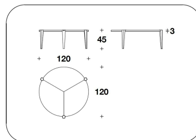
TCT (CF60P/1) - TCT (CF60E/1) - TCT (CF60PM/1) - TCT (CF60EM/1) COFFEE TABLE Ø 120x45H.cm Ø 47 1/3x17 3/4H."
