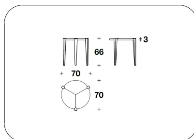
TCT (CF61P/2) - TCT (CF61E/2) - TCT (CF61PM/2) - TCT (CF61EM/2) SIDE TABLE Ø 70x66H.cm Ø 27 2/3x26H."
